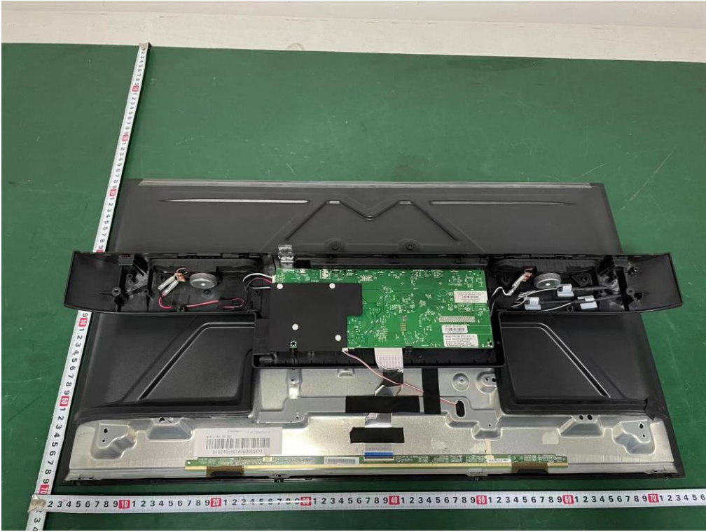
Internal photos M/N: TC-LE32K-AN2401
