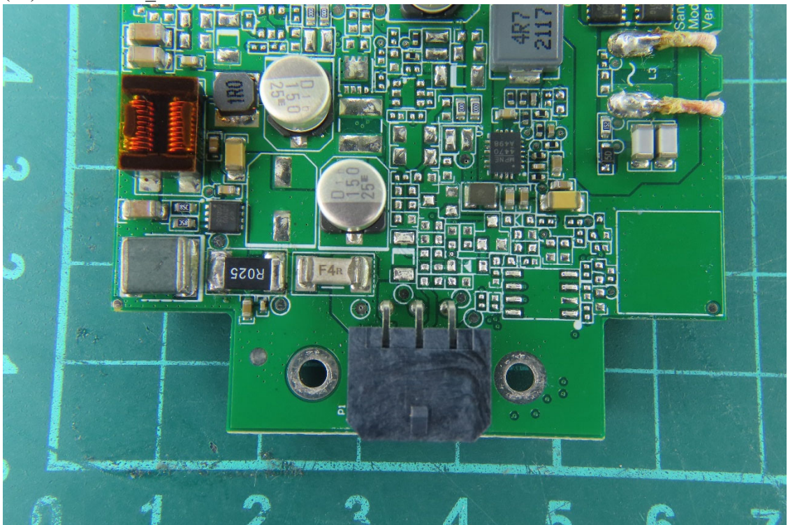
(24) EUT Photo_M/N: 240000-01-202
