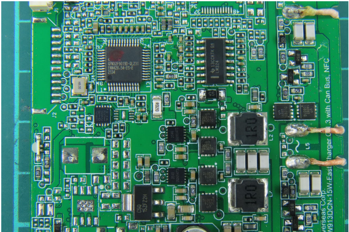
(23) EUT Photo_M/N: 240000-01-202
