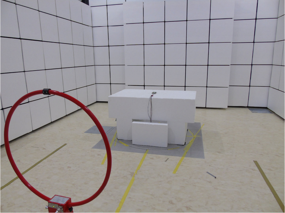
Loop Antenna
