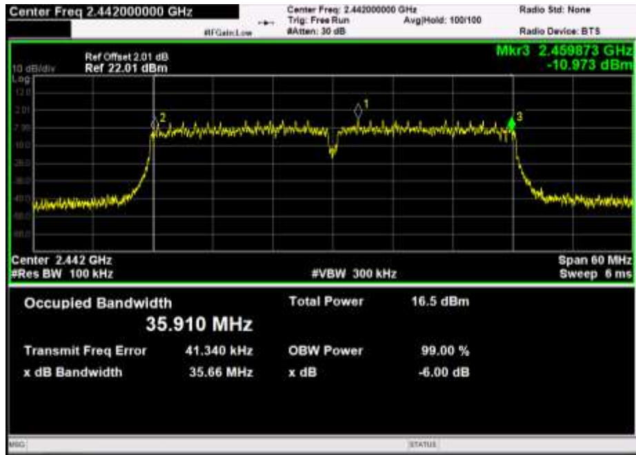
Channel 7:2.442GHz:
