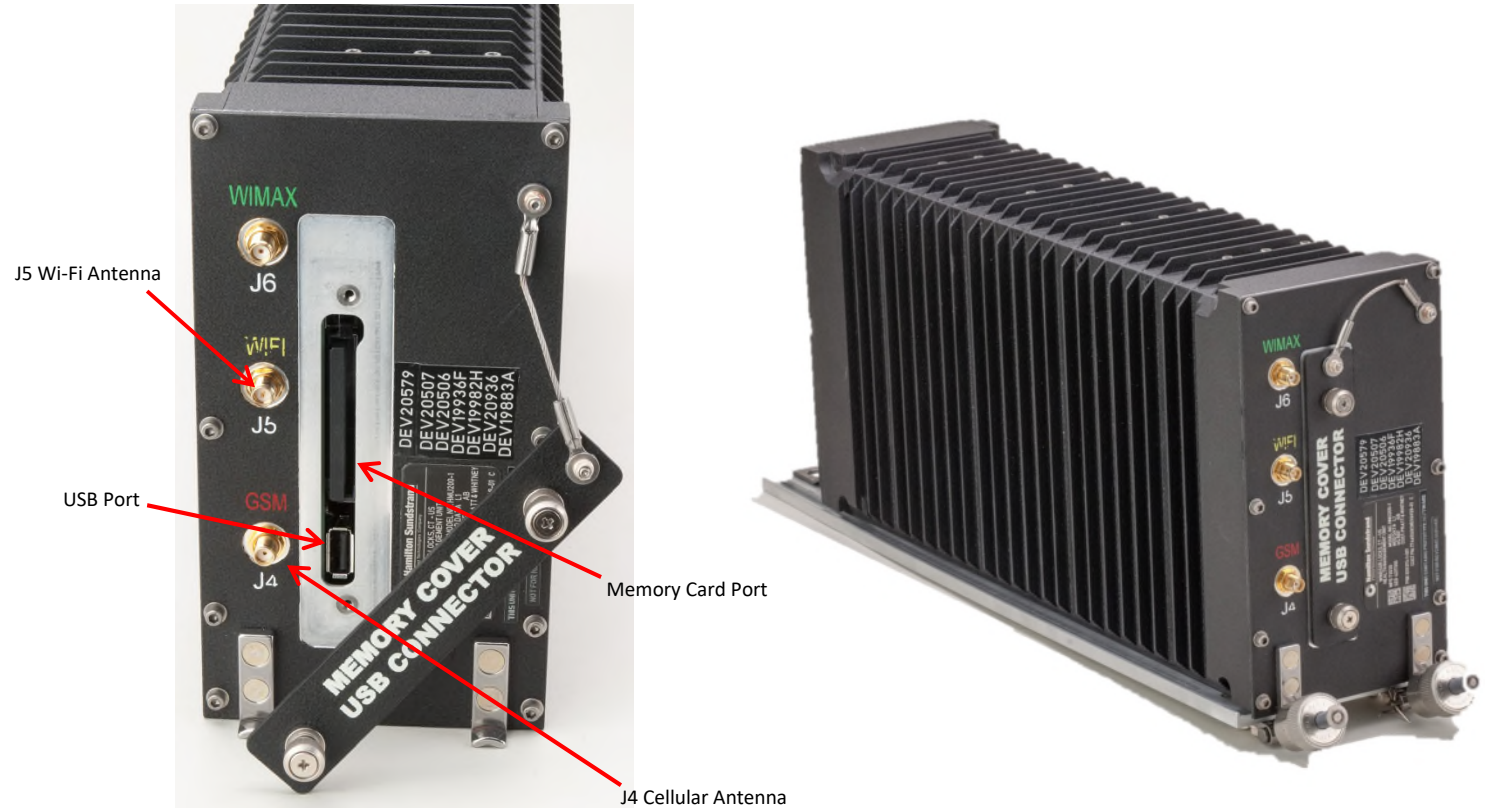
Figure 1: Isometric View of eFAST product on mounting tray (as installed in aircraft)
