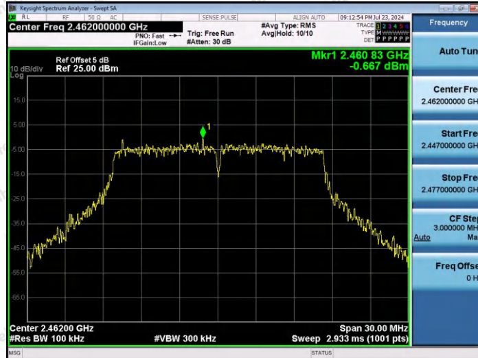
11G-Ant1-2462-0~Reference-PASS
