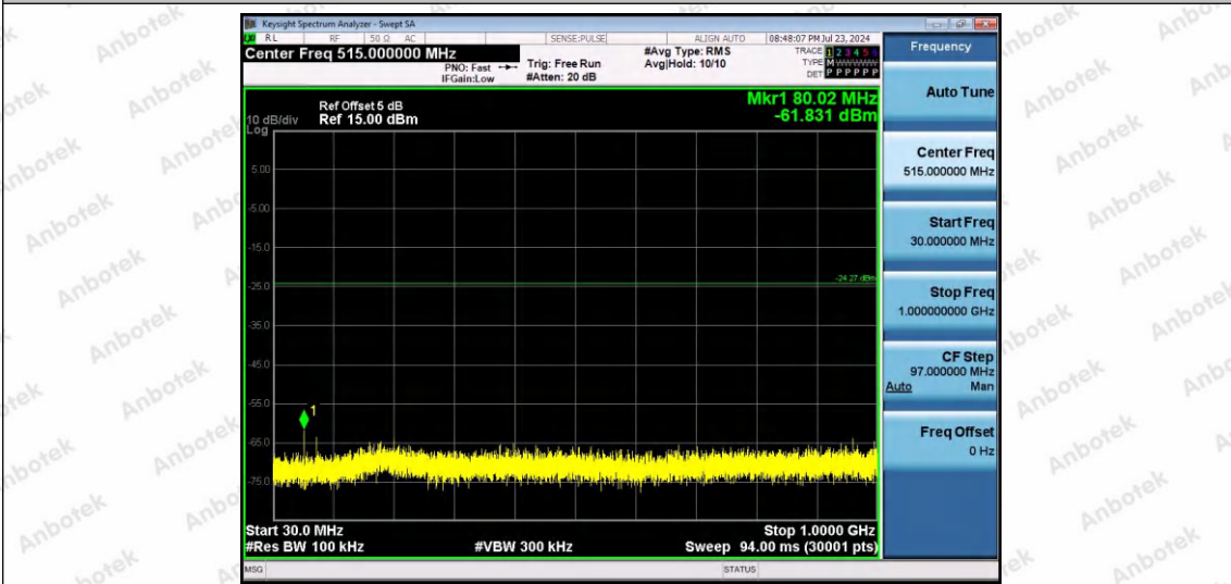
11B-Ant1-2412-30~1000-PASS
