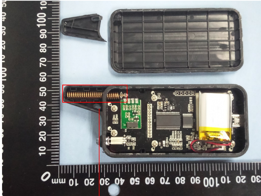
433MHz Antenna
