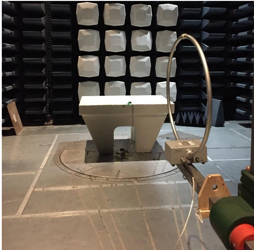
Radiated Emissions 3m SAC 1 – 150kHz – 30MHz – Photo1
