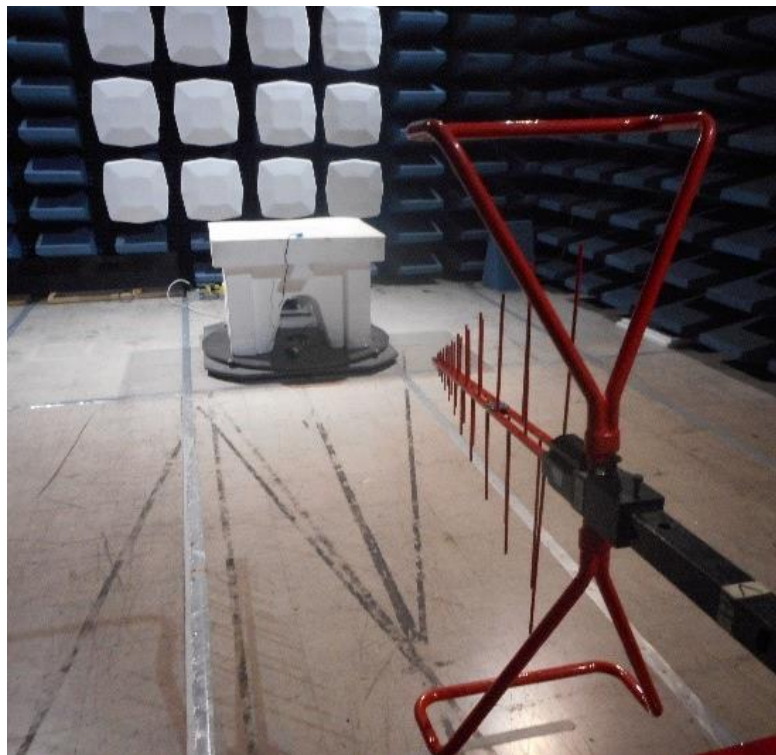
Radiated Emissions 3m SAC 30MHz – 1GHz – Photo1
