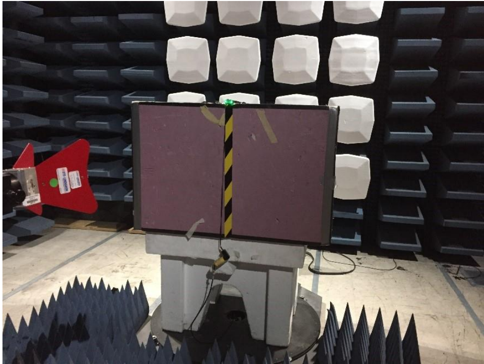
Radiated Emissions 3m SAC 1 – 18GHz – Photo1
