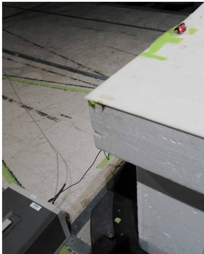
AC Conducted Emissions 3m SAC – Photo2
