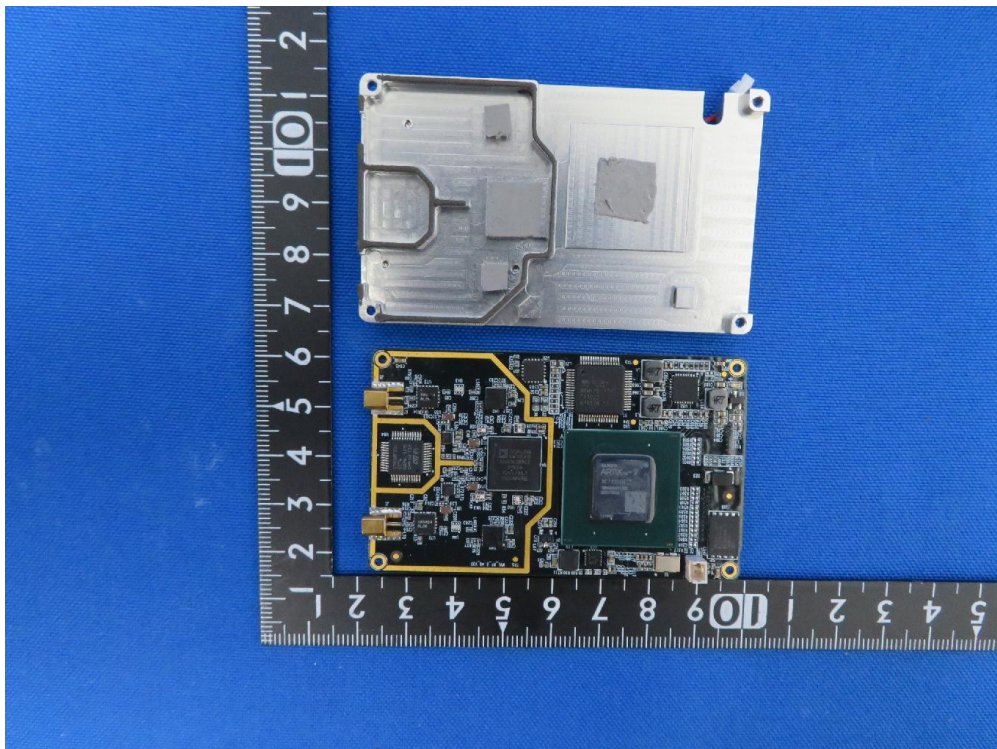
(2) EUT Photo (Model: WLN210-BM-b)
