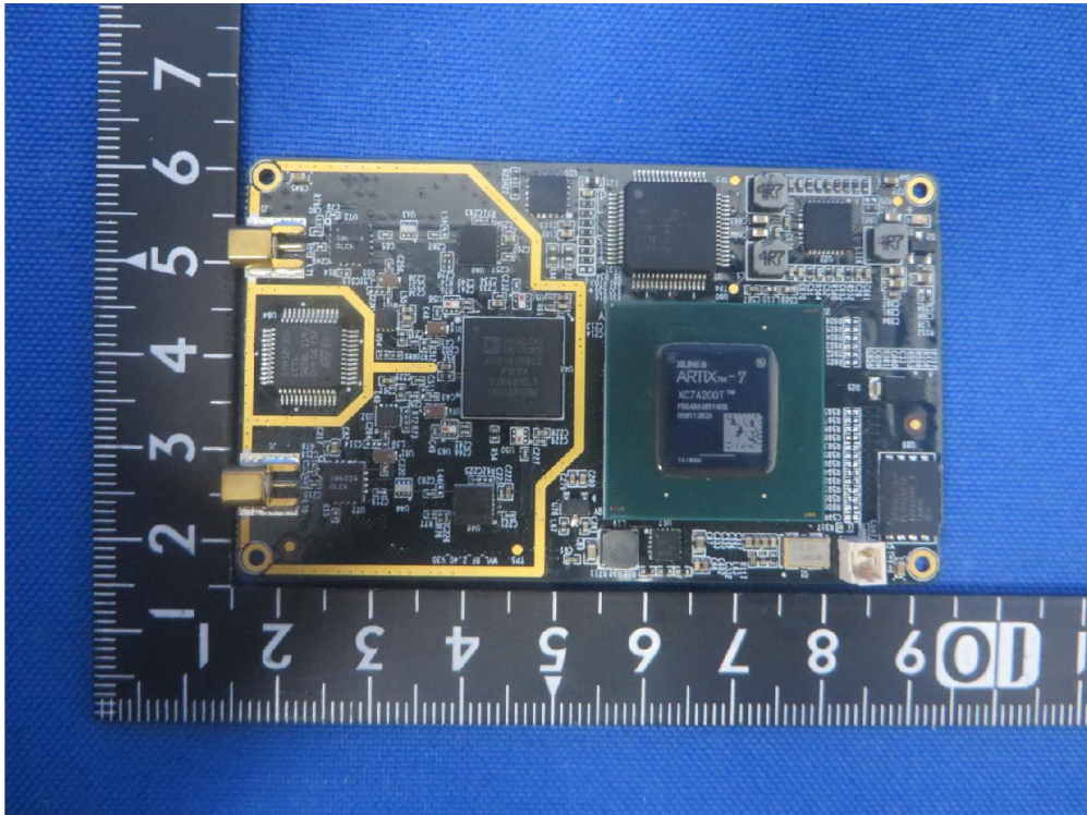
(5) EUT Photo (Model: WLN210-BM-d)
