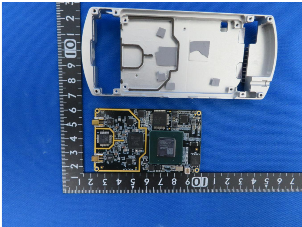
(4) EUT Photo (Model: WLN210-BM-d)
