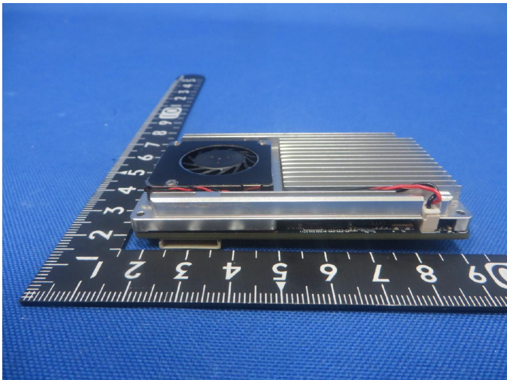
(8) EUT Photo (Model: WLN210-BM-b)
