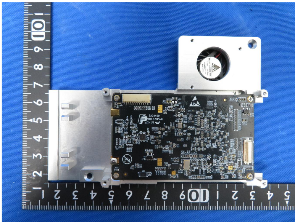
(12) EUT Photo (Model: WLN210-BM-c)
