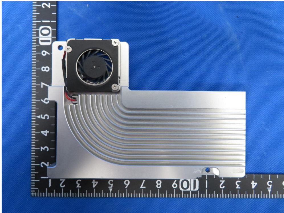
(11) EUT Photo (Model: WLN210-BM-c)
