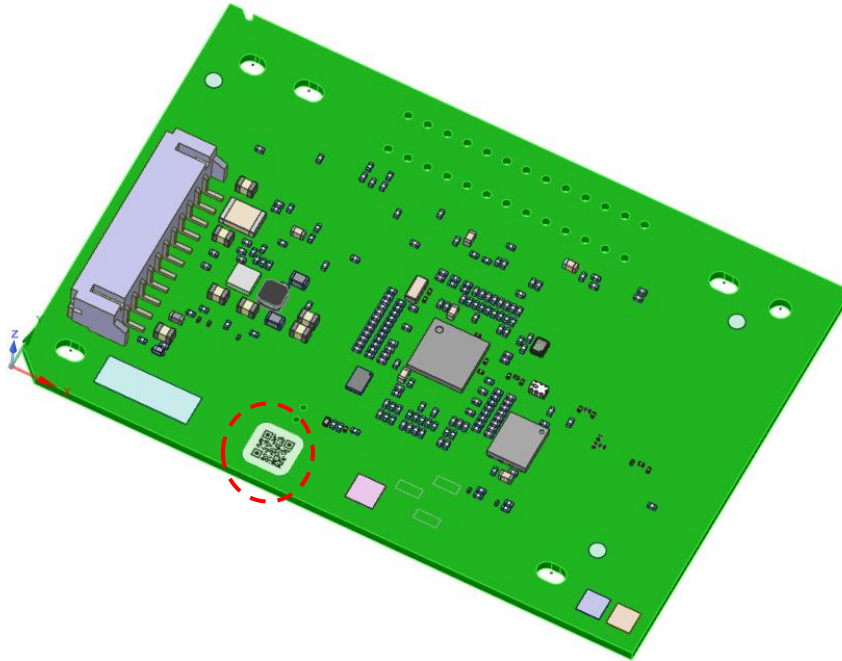
Figure 2 EHRMODULE – top sticker placement
