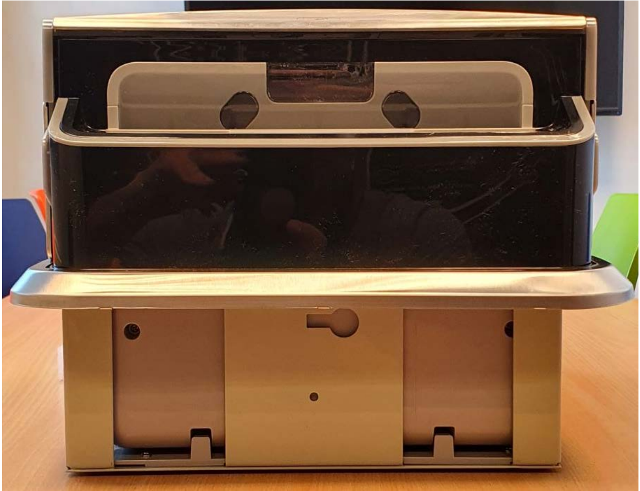
Figure 12: EHTRECCSD Host Bottom View
