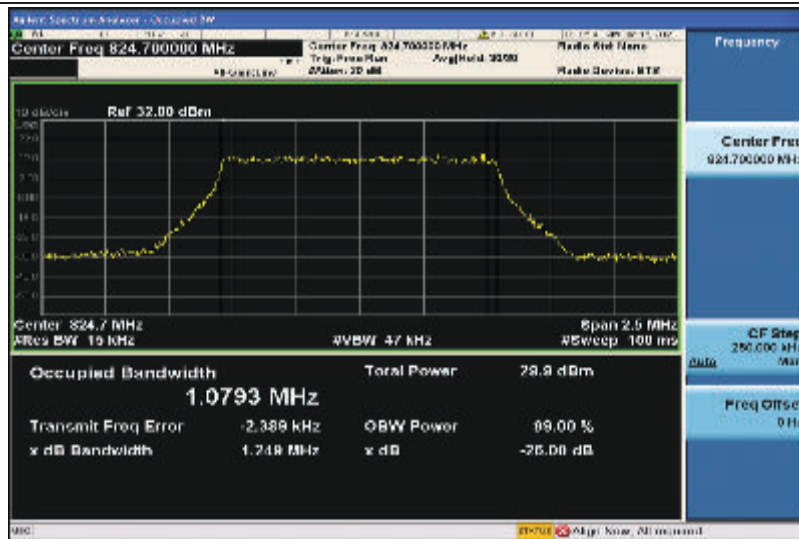
Band5-1.4MHz-QPSK-20407-6RB#0-1.0793
