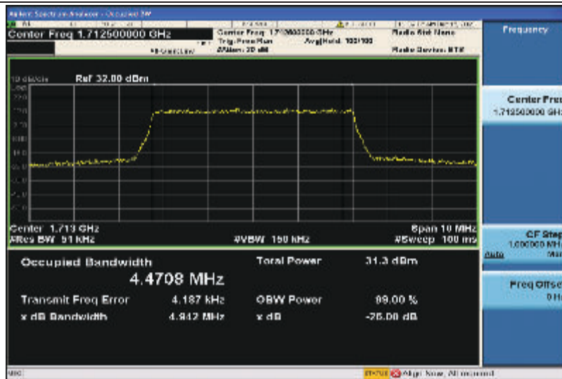
Band4-5MHz-QPSK-19975-25RB#0-4.4708
