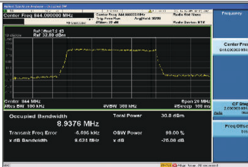
Band5-10MHz-16QAM-20600-50RB#0-8.9376
