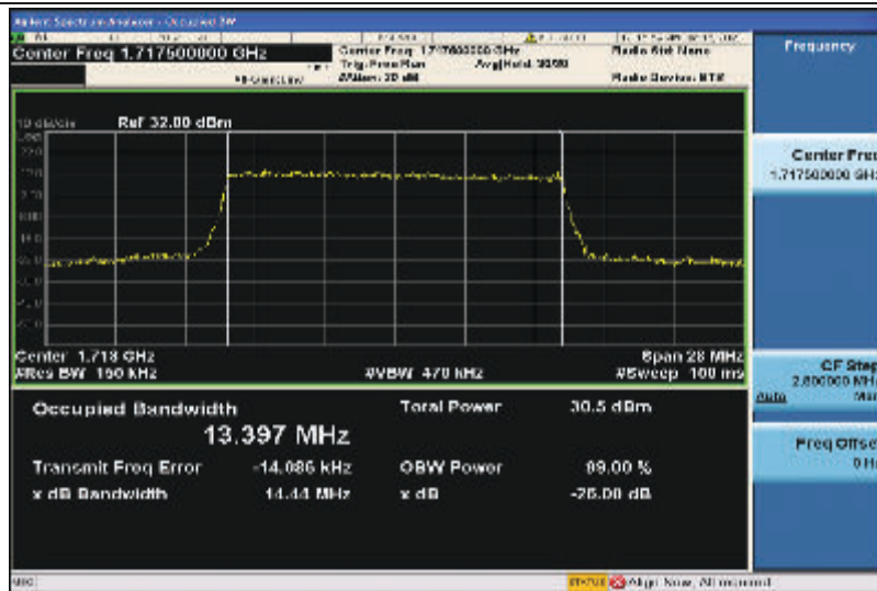
Band4-15MHz-16QAM-20025-75RB#0-13.397
