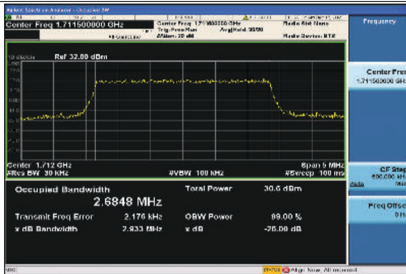
Band4-3MHz-QPSK-19965-15RB#0-2.6848
