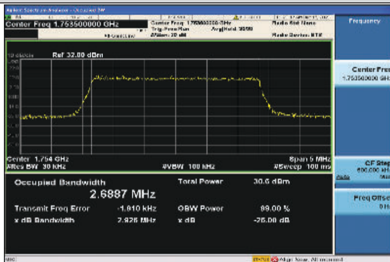
Band4-3MHz-QPSK-20385-15RB#0-2.6887
