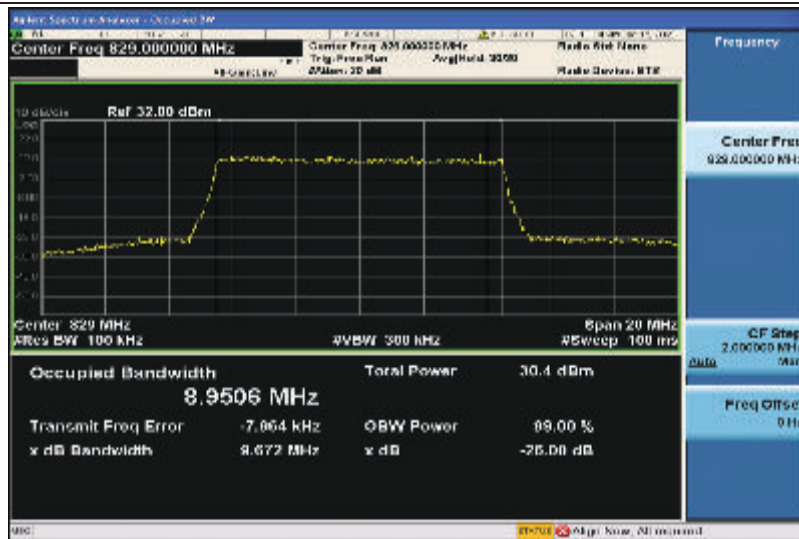
Band5-10MHz-16QAM-20450-50RB#0-8.9506
