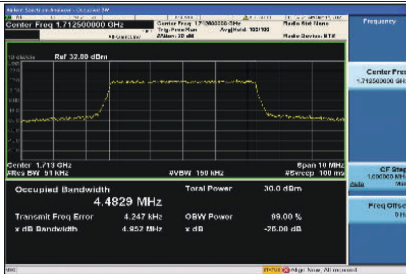
Band4-5MHz-16QAM-19975-25RB#0-4.4829
