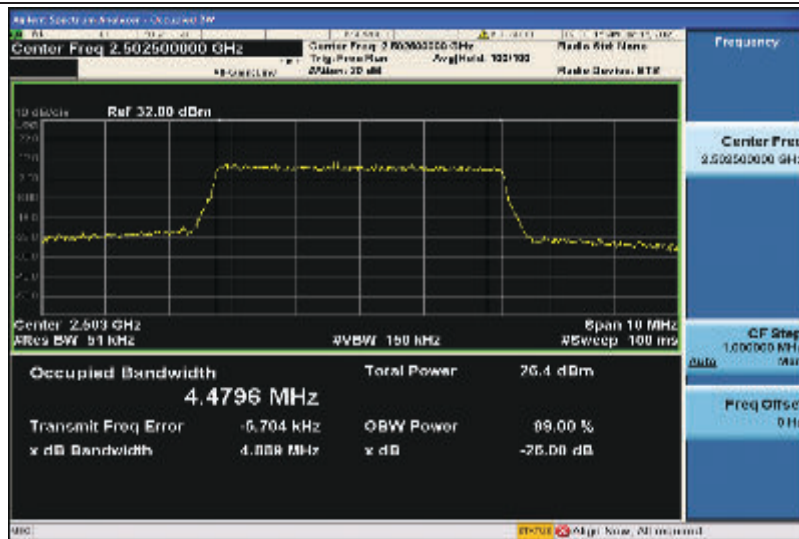
Band7-5MHz-16QAM-20775-25RB#0-4.4796
