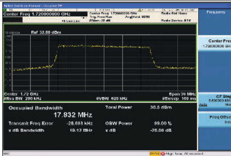
Band4-20MHz-16QAM-20050-100RB#0-17.832
