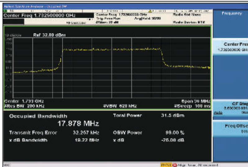
Band4-20MHz-QPSK-20175-100RB#0-17.878
