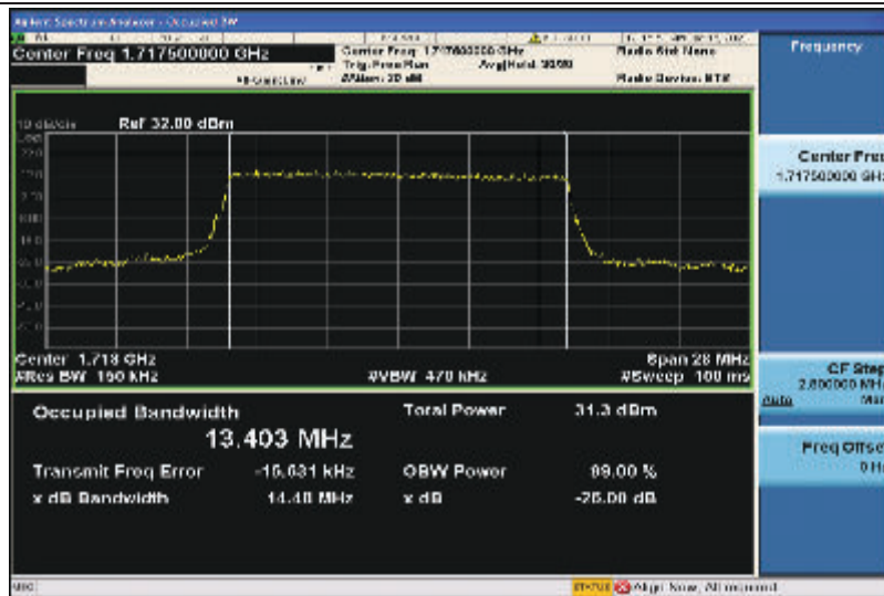
Band4-15MHz-QPSK-20025-75RB#0-13.403
