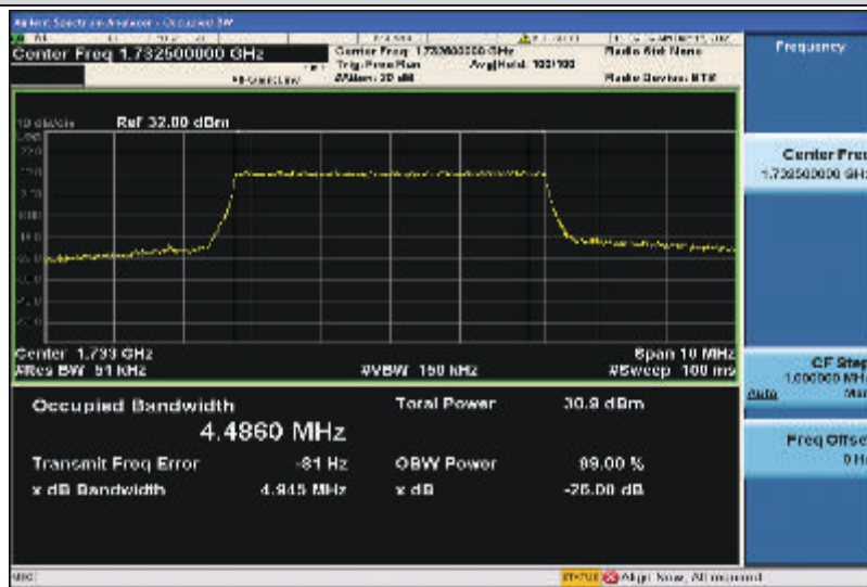
Band4-5MHz-QPSK-20175-25RB#0-4.4860
