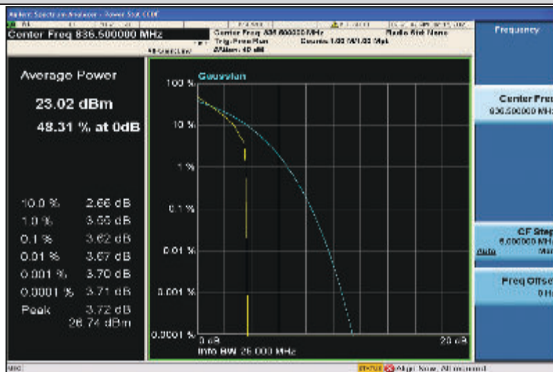
Band5-10MHz-QPSK-20525-1RB#0
