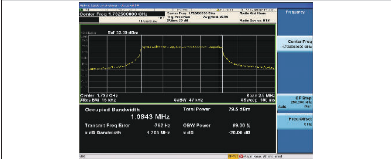
Band4-1.4MHz-QPSK-20175-6RB#0-1.0843
