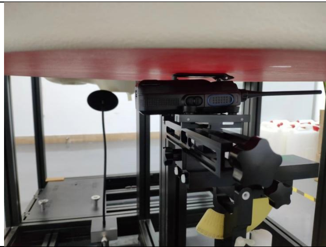
Body-worn(0mm) Type D
