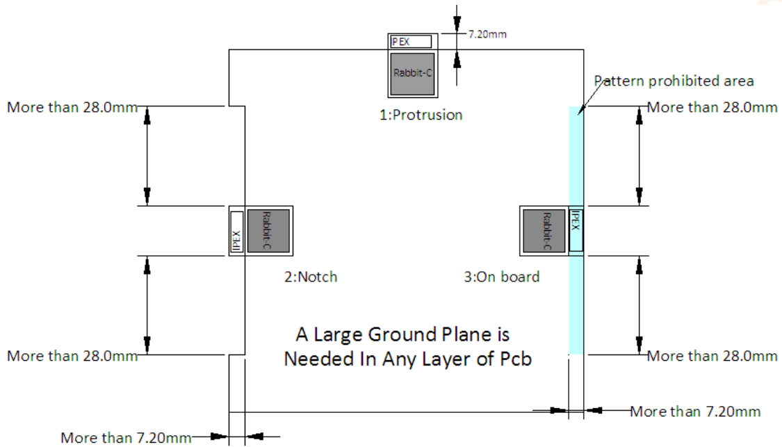
Figure 2: Module Placement
