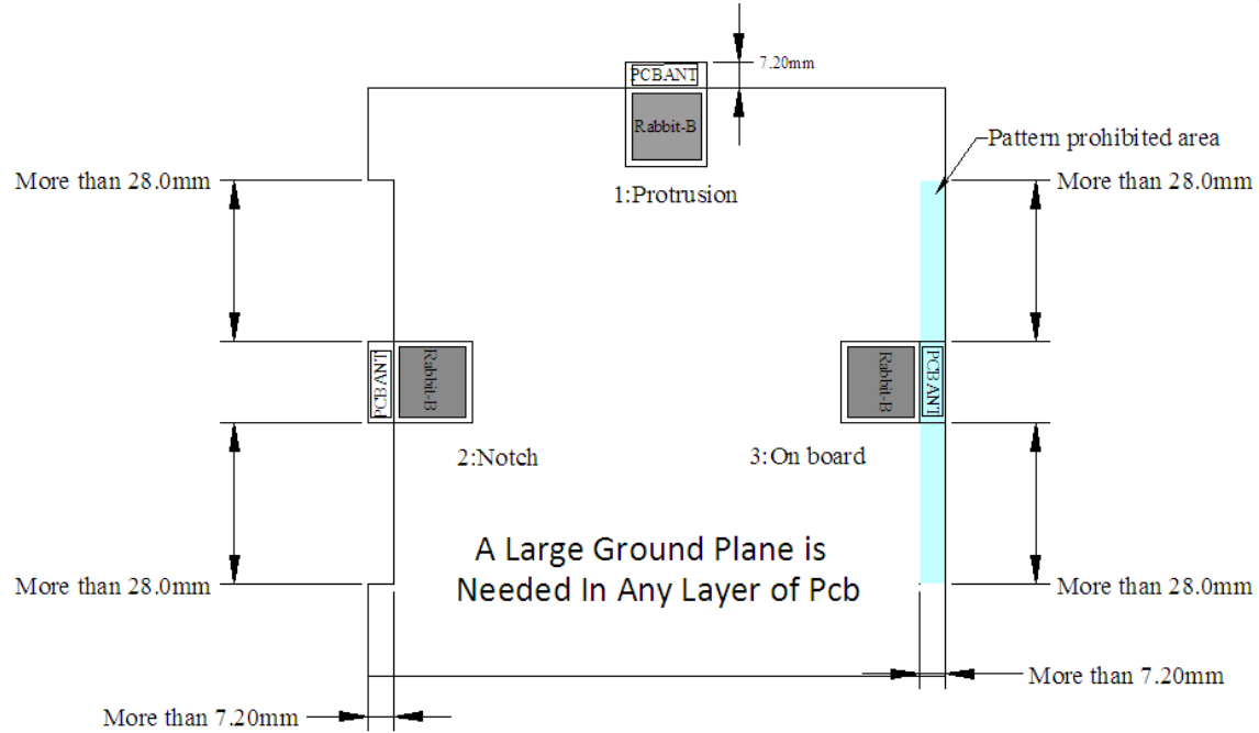
Figure 2: Module Placement
