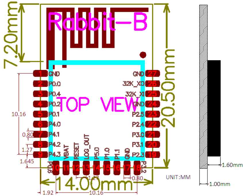
Figure 2: Mechanical Information
