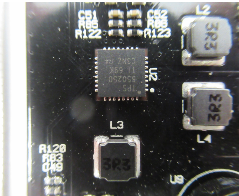
EUT –Chip View-2
