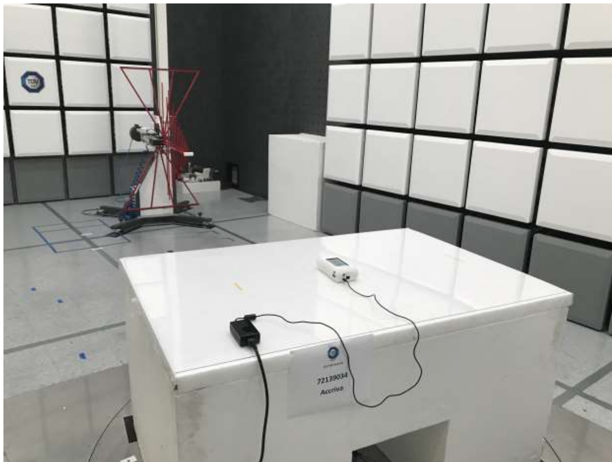
Radiated Emissions Test Setup (below 1000MHz)
