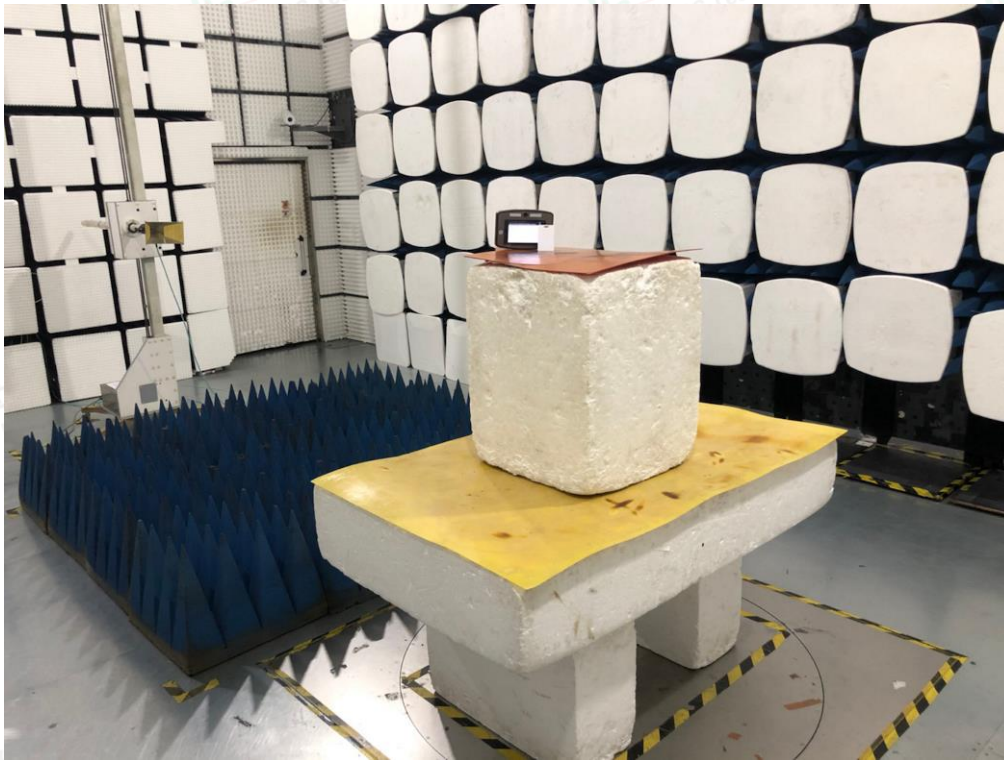
Fig. 3 Test Setup Photo of Line Conducted Emissions Measurement
