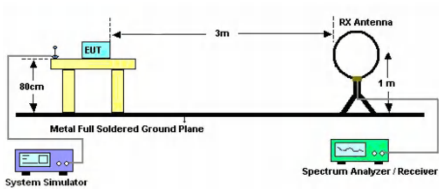
Figure 2. 30MHz to 1GHz
