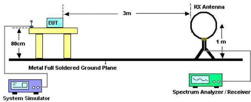
Figure 2. 30MHz to 1GHz
