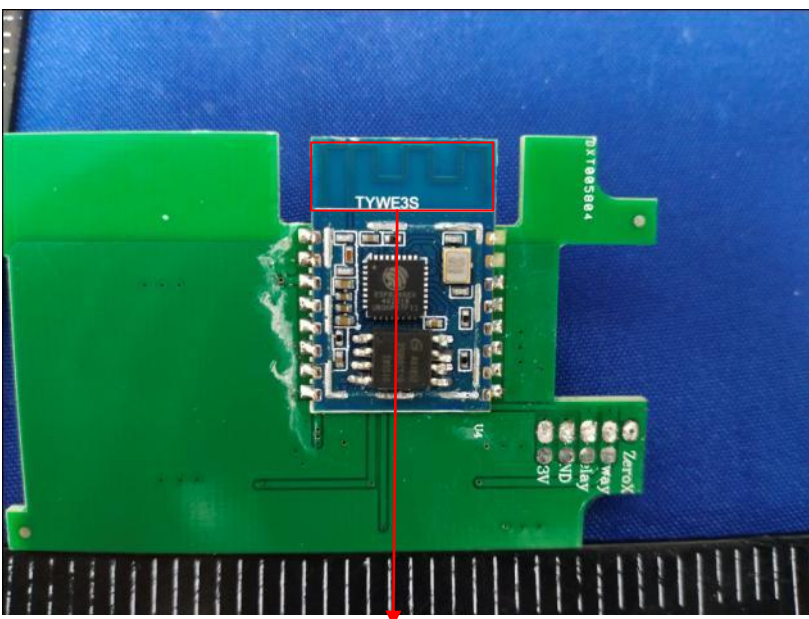
RF Antenna
