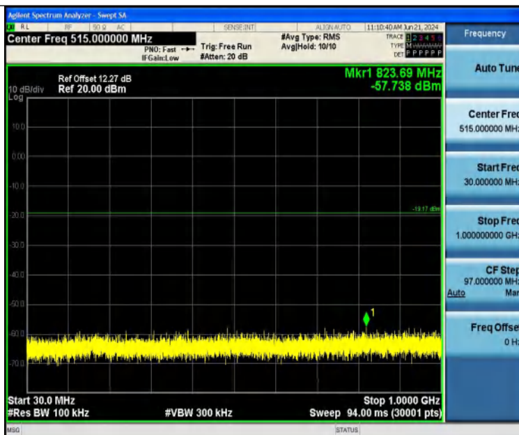
11B-Ant1-2437-30~1000-PASS
