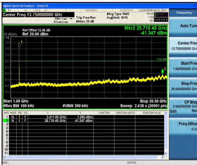
11B-Ant1-2412-1000~26500-PASS
