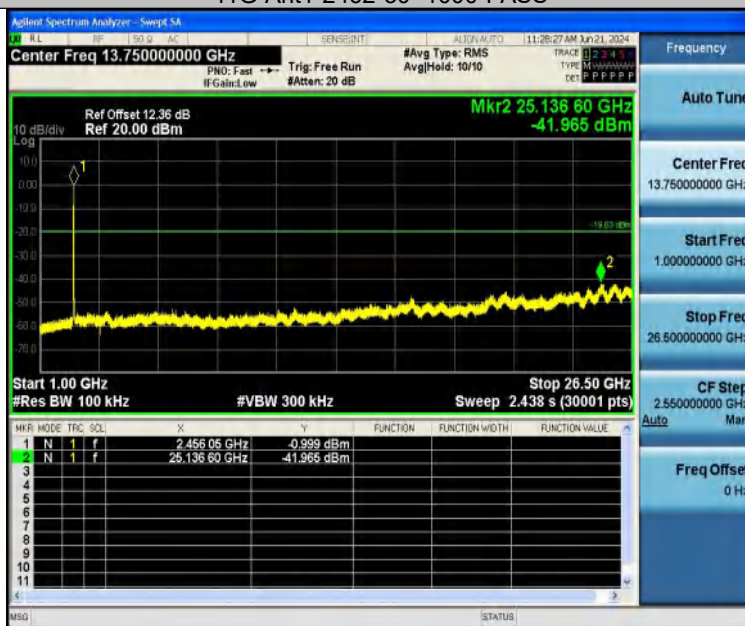
11G-Ant1-2462-1000~26500-PASS
