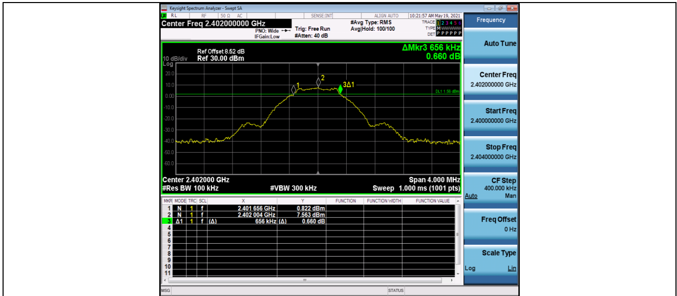
BLE_BT4.0_Ant1_2402
