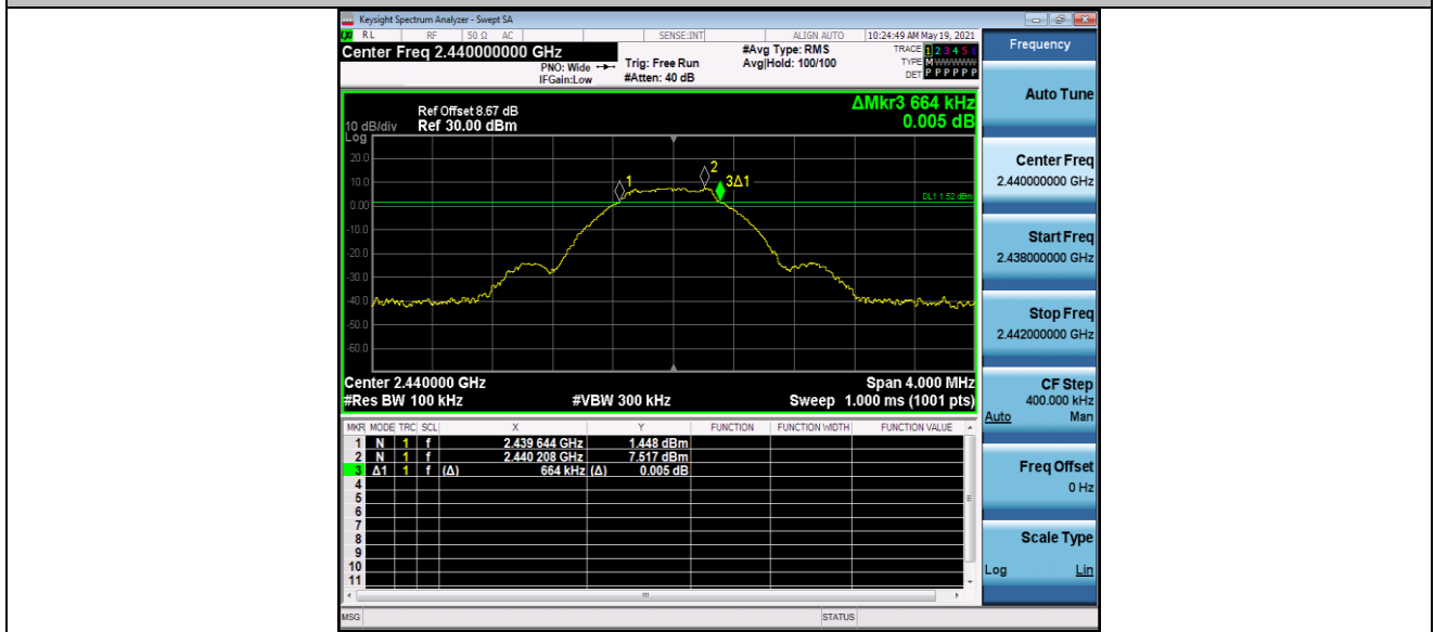
BLE_BT4.0_Ant1_2440
