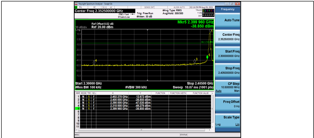
BLE_1M_Ant1_Low_2402
