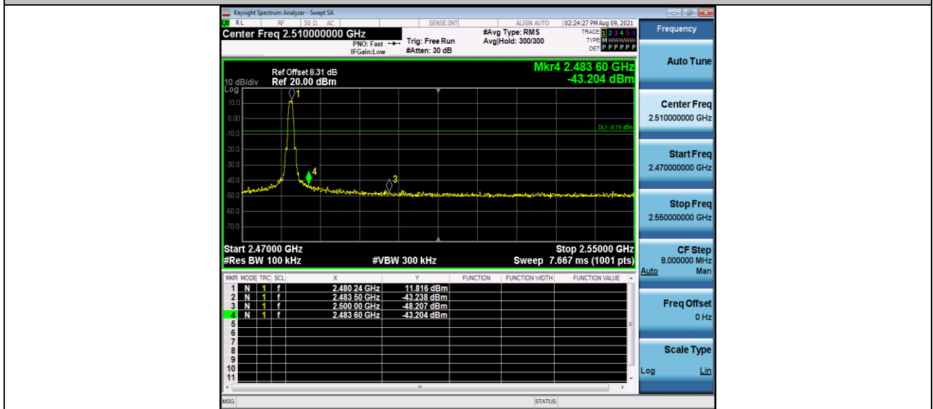
BLE_1M_Ant1_High_2480
