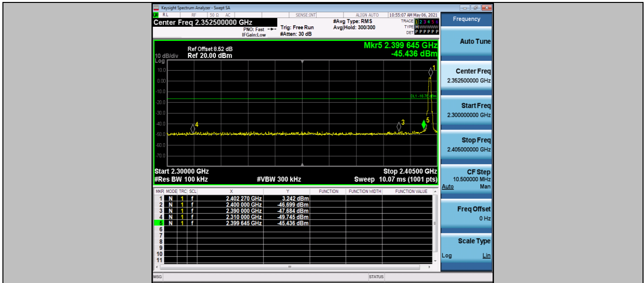
BLE_BT4.2_Ant1_Low_2402
