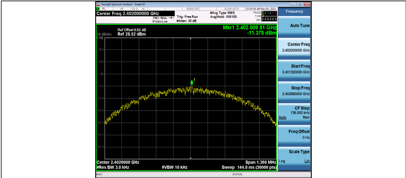
BLE_BT4.2_Ant1_2402
