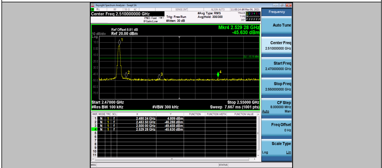
BLE_BT4.2_Ant1_High_2480
