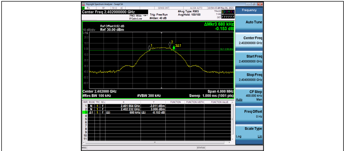
BLE_BT4.2_Ant1_2402
