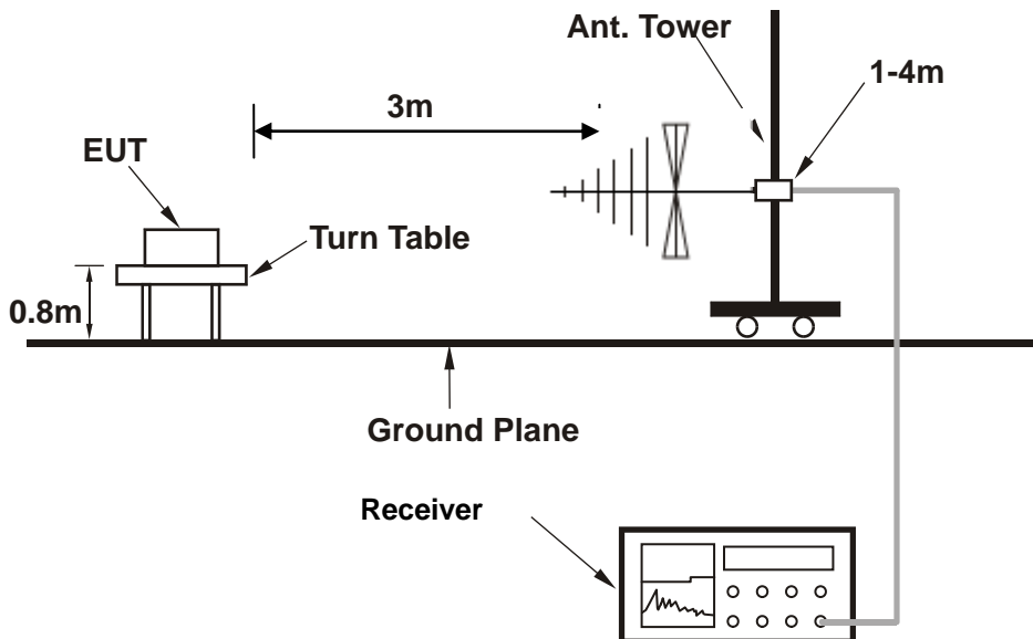
Setup diagram for Radiation(Below 1G) Test
