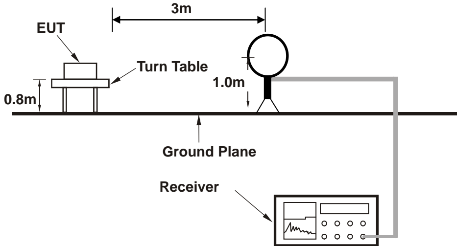
Setup diagram for Radiation(Below 1G) Test
