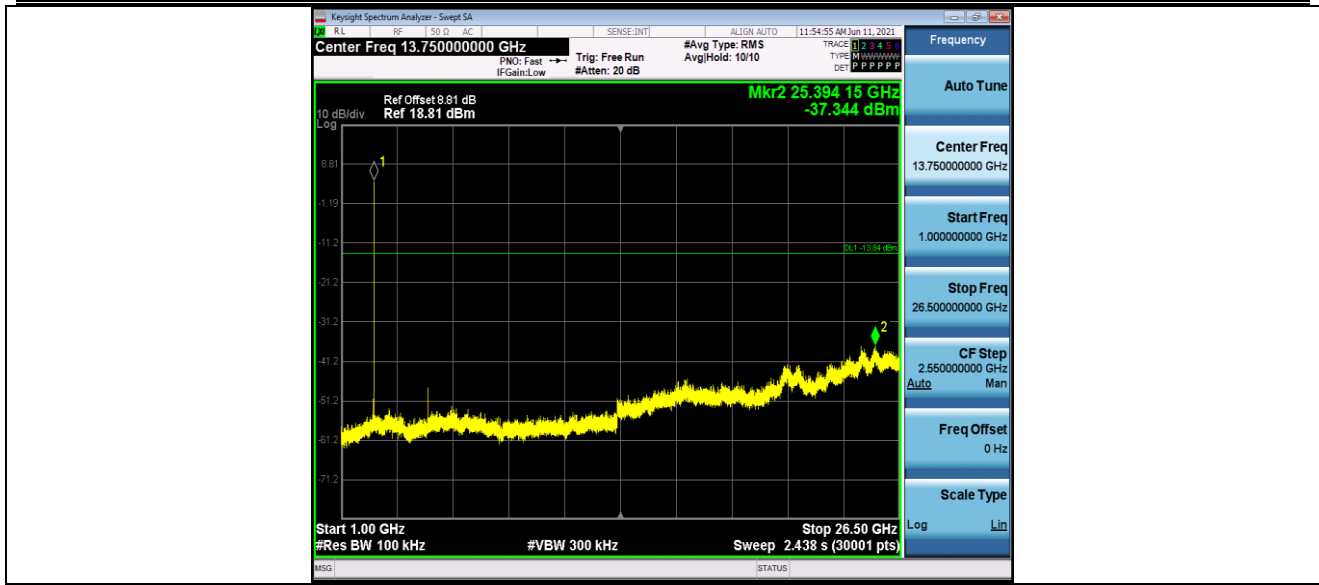
BLE_BT4.2_Ant1_2480_1000~26500
