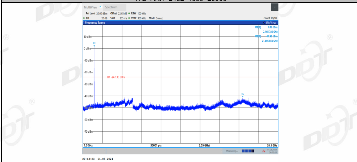
11N20SISO_Ant1_2412_0~Reference
