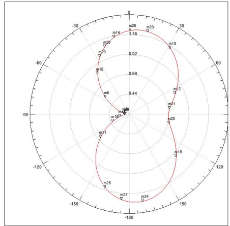
Radiation Pattern 1
