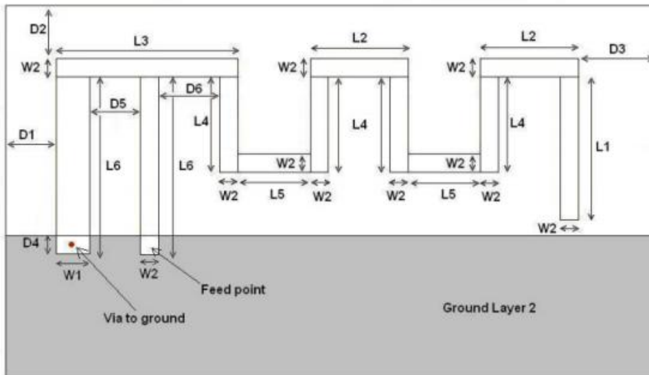
Figure 3: Antenna Dimensions
