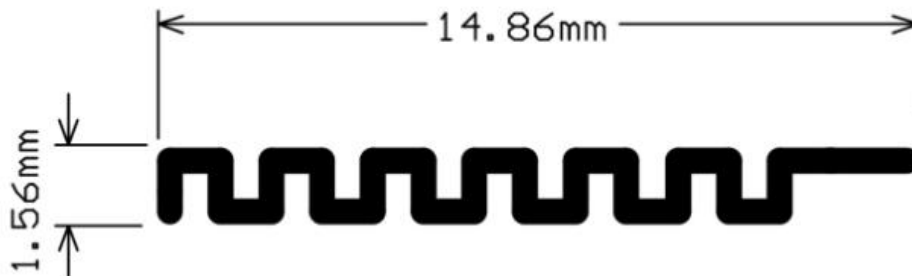
Antenna Photo & Length (mm)
