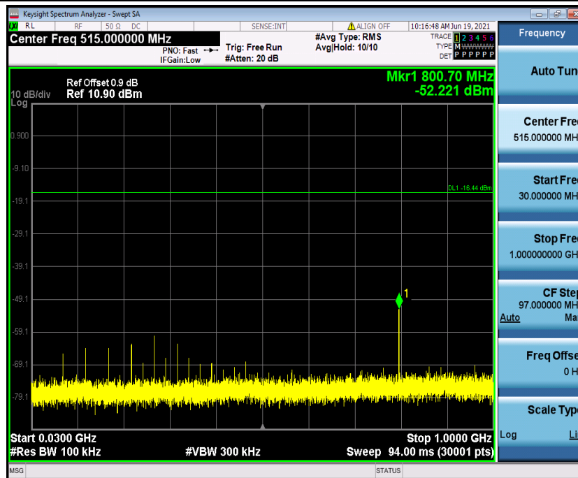
3DH5_Ant1_2402_30~1000
