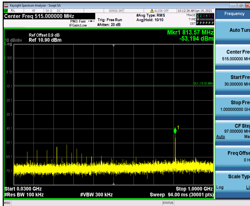
2DH5_Ant1_2441_30~1000
