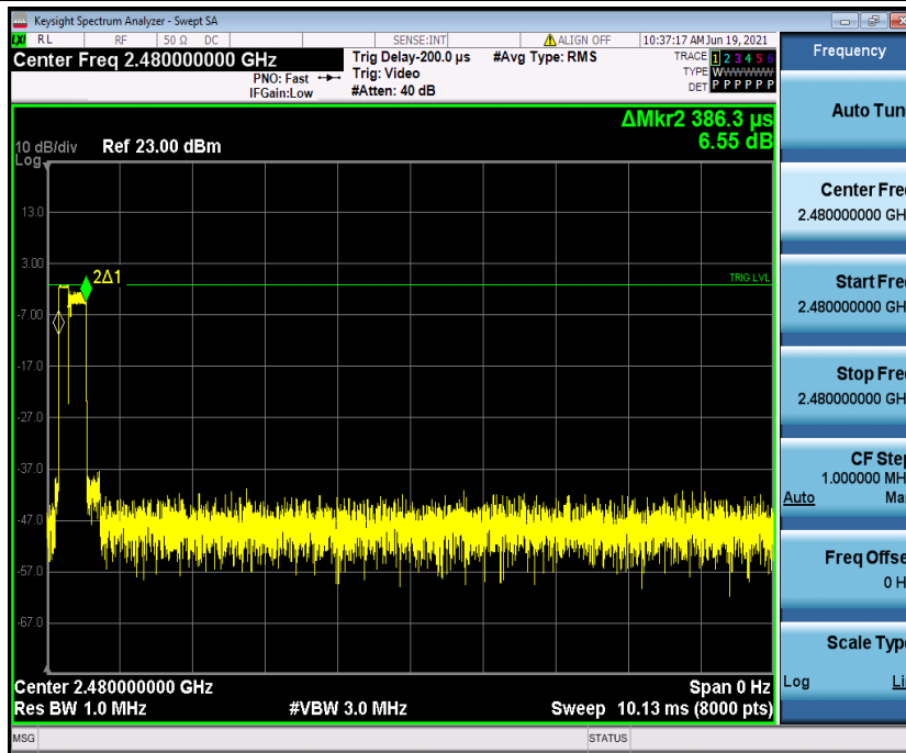
2DH1_Ant1_Hop_2480
