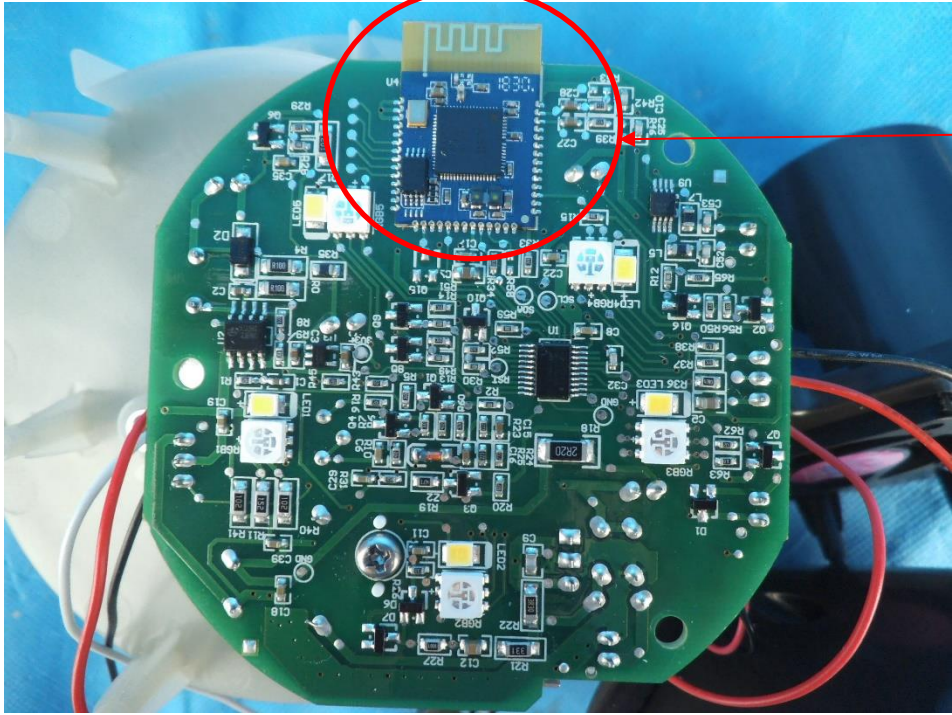
RF Antenna
