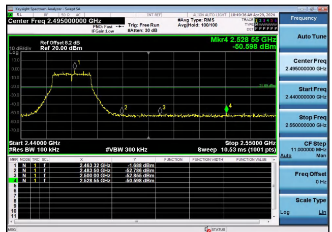
Right bandedge
