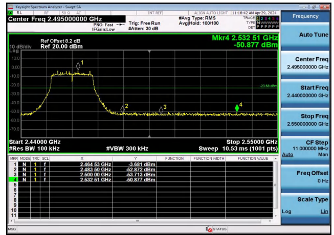
Right bandedge
