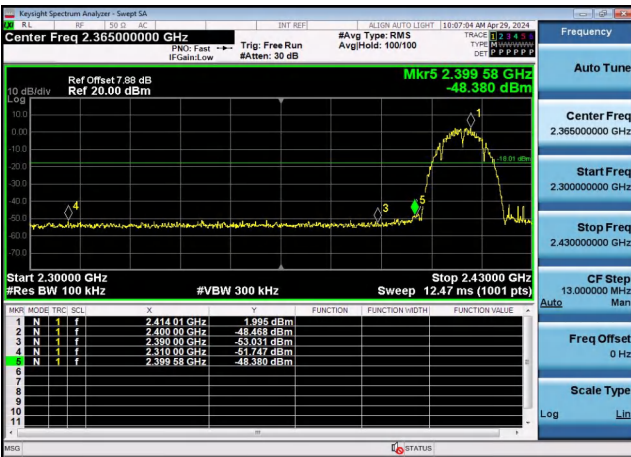
Left bandedge
