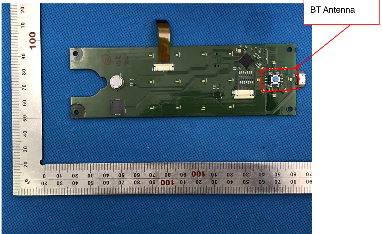
INTERNAL VIEW OF EUT 4
