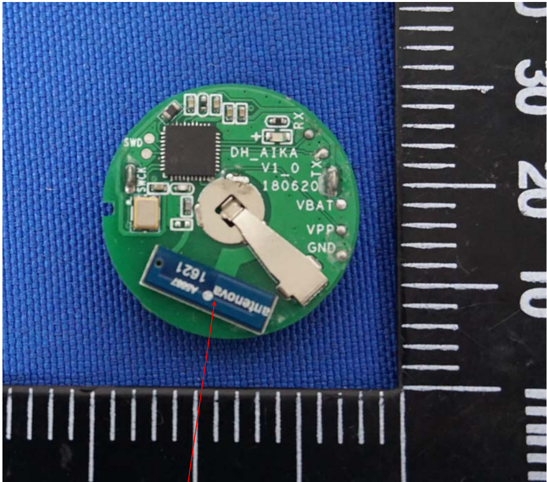
Chip antenna
