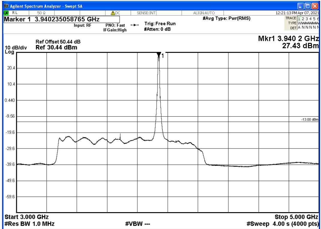
Antenna A, 5G Modulation QPSK - Carrier Bandwidth 10.0 MHz - Channel Position Top: 3945 MHz – Range 3GHz to 5G
