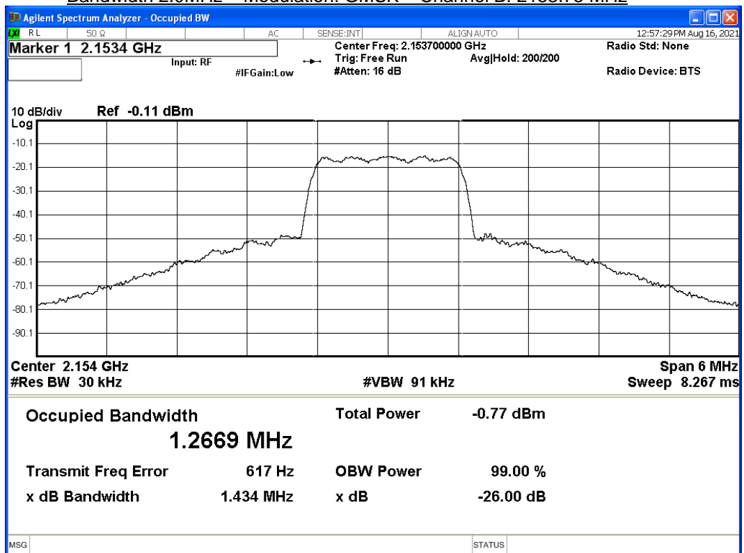
Bandwidth 2.0MHz – Modulation: GMSK – Channel B: 2153.75 MHz
