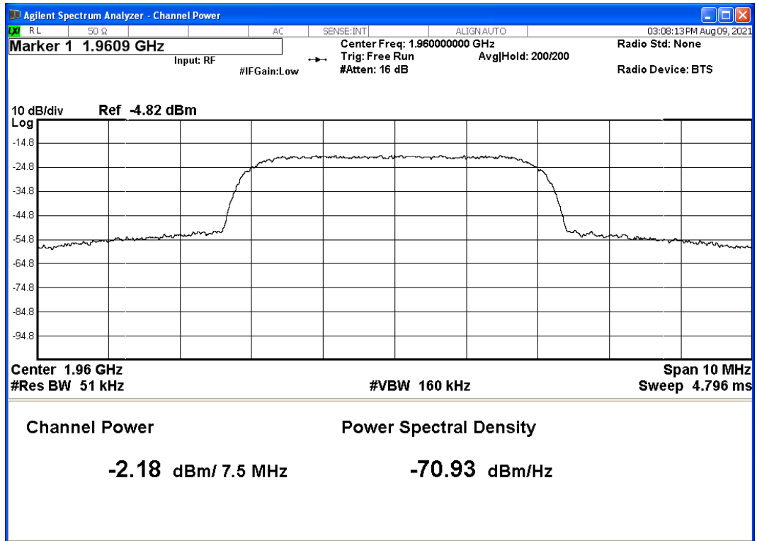
Graph 2: Output Power – Port 1B – Middle Channel
