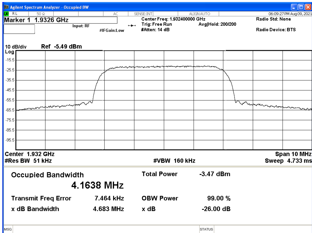
Bandwidth 5.0MHz – Modulation: QPSK – Channel B: 1932.4 MHz
