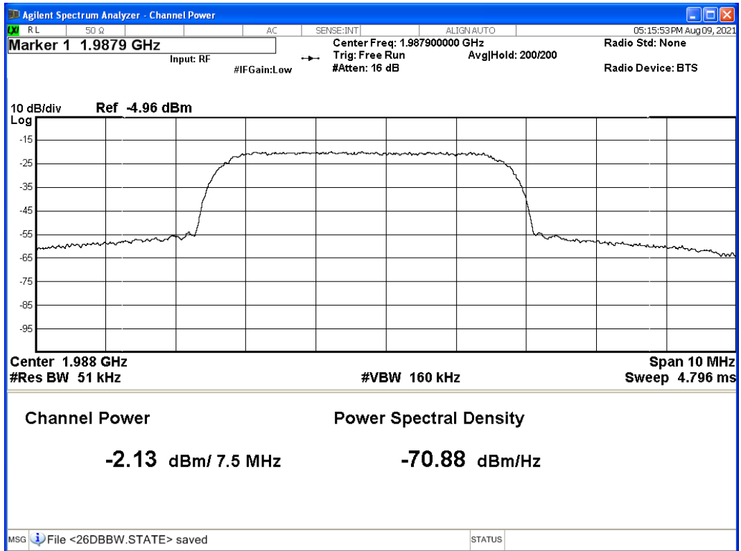
Graph 3: Output Power – Port 1B – Top Channel
