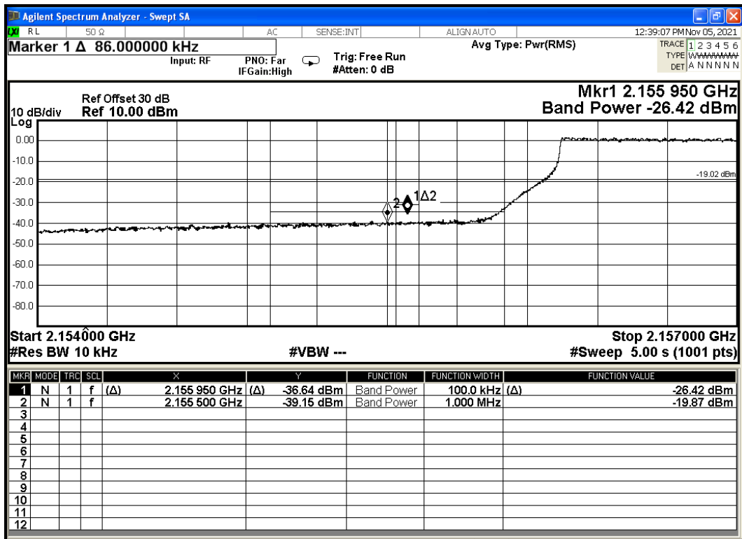
Modulation QPSK - Carrier Bandwidth 5.0 MHz – Top – Channel Position: 2155MHz (Band Power 100kHz and 1MHz)
