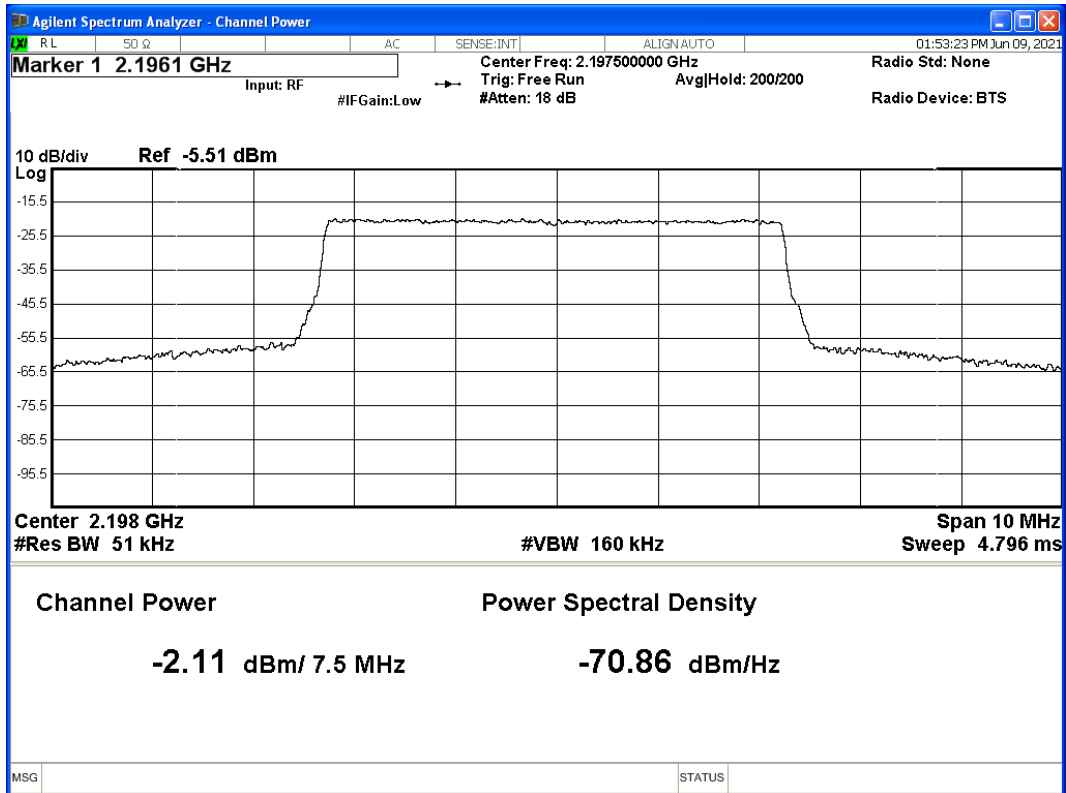
Graph 5: Output Power – Port 2B – Channel: 2197.5 MHz
