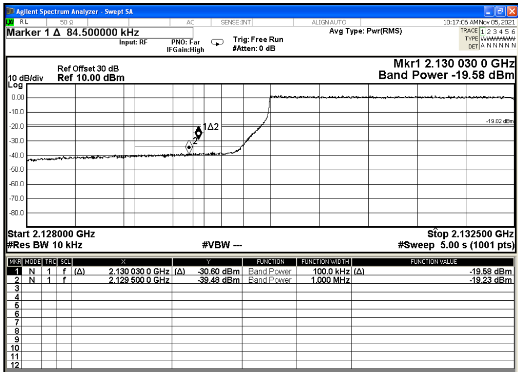
Modulation QPSK - Carrier Bandwidth 5.0 MHz – Top of the Band – Channel Position: 2132.5 MHz (Band Power 100kHz & 1MHz)
