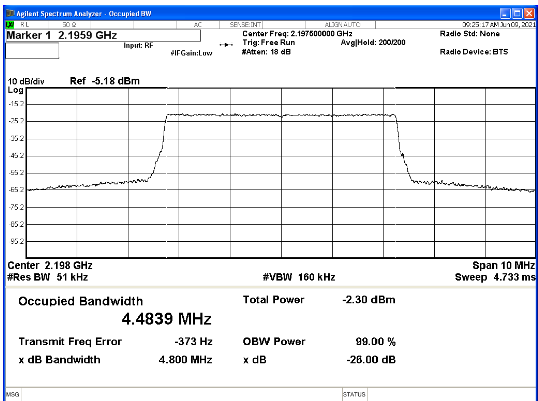
Bandwidth 5.0MHz – Modulation: QPSK – Channel Top: 2197.5 MHz
