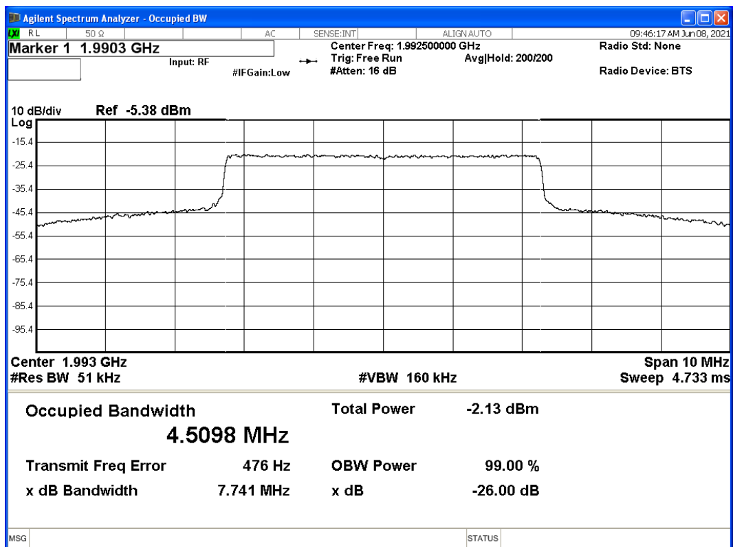
Bandwidth 5.0MHz – Modulation: QPSK – Channel Top: 1992.5 MHz
