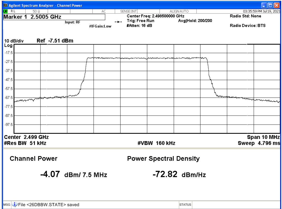
Graph 1: Output Power – Port 2A – Bottom Channel: 2498.5 MHz
