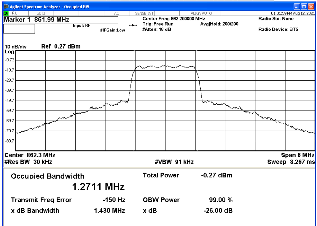
Bandwidth 2.0MHz – Modulation: QPSK – Channel Middle: 862.25 MHz
