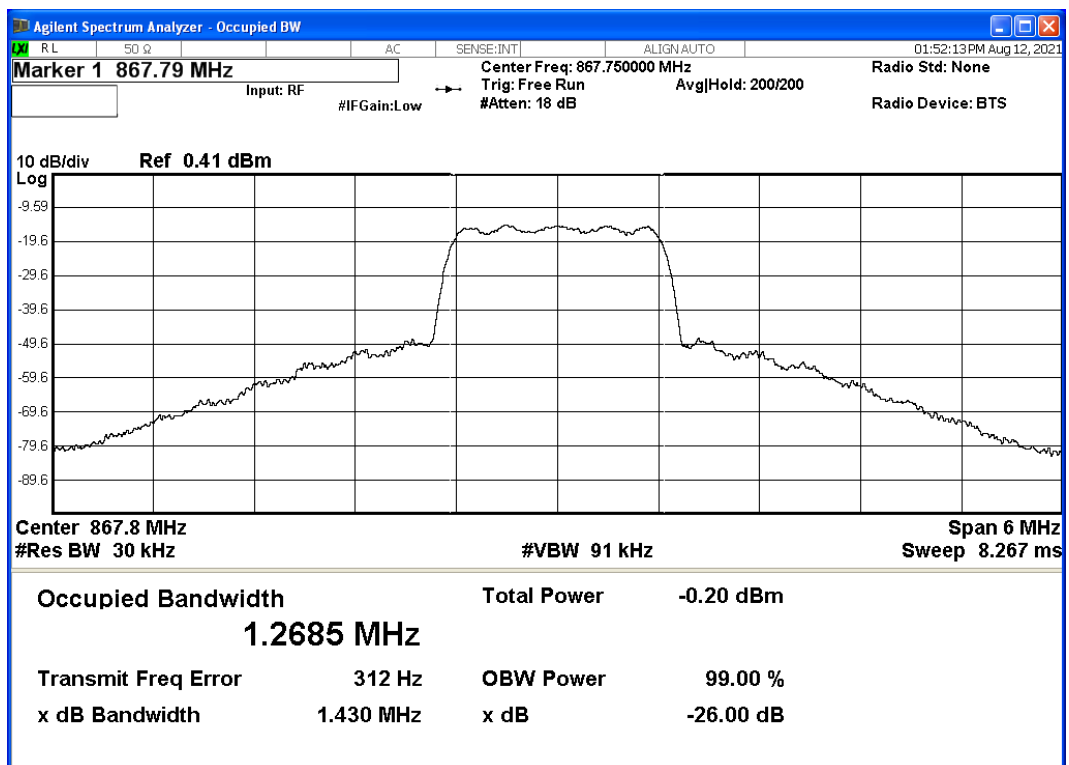
Bandwidth 2.0MHz – Modulation: QPSK – Channel Top: 867.75 MHz
