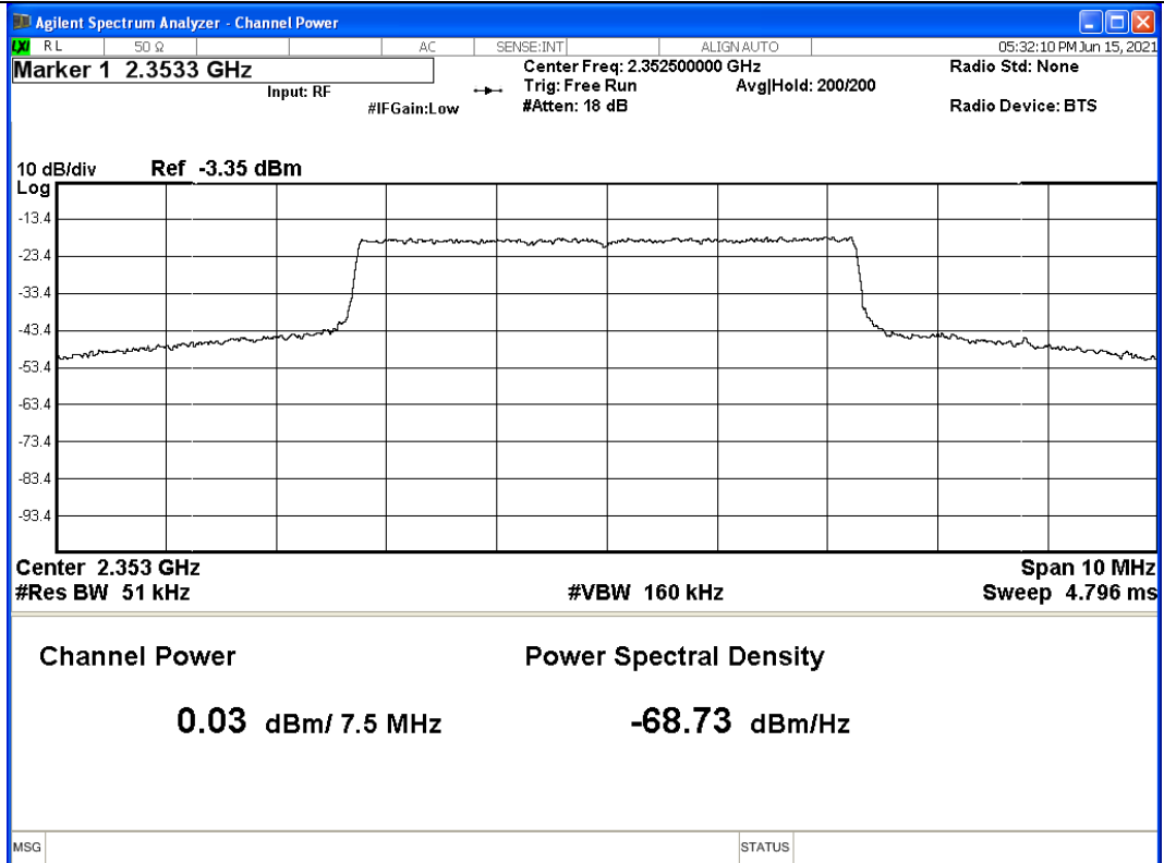
Graph 1: Output Power – Port 2A in dBm/7.5MHz
