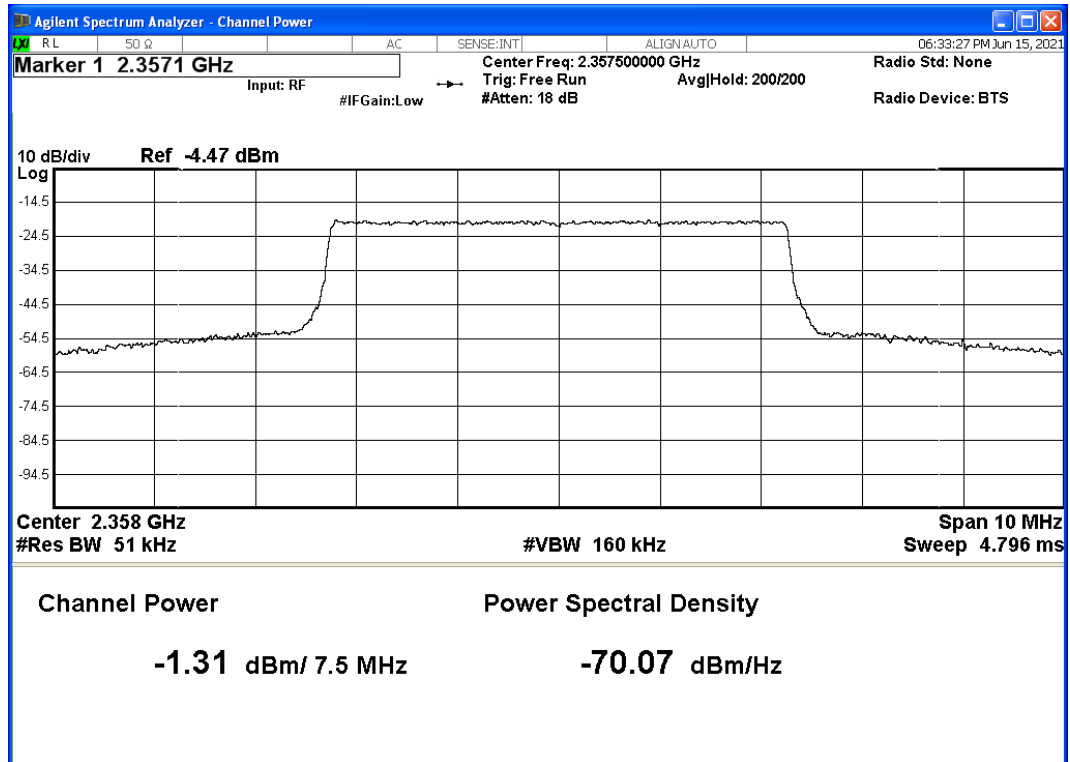
Graph 3: Output Power – Port 1B – Top Channel
