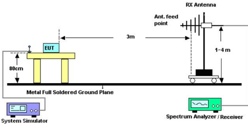
Radiated Emission Test-Setup Frequency 30MHz-1000MHz
