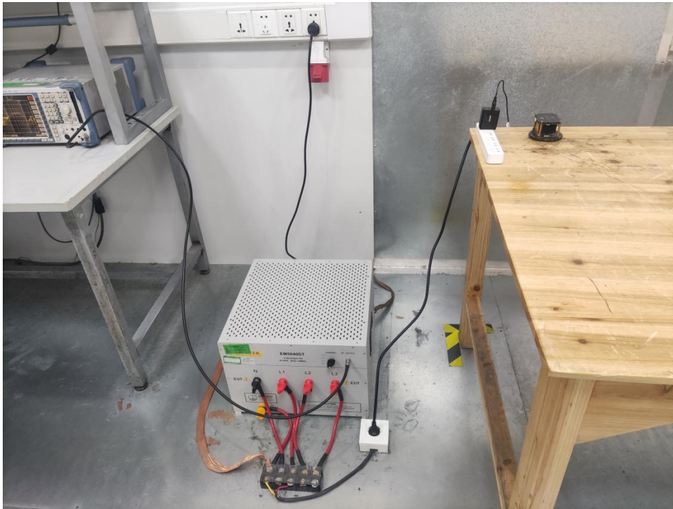
FCC ID: 2AQRPTJC109AWC Photo of Conducted Emission Measurement
