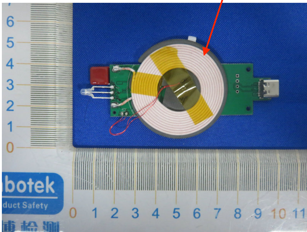
Coil Antenna
