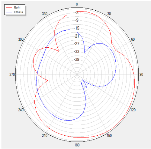
H Theta=90 freq=820MHz
