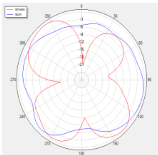
V Phi=0 freq=1575MHz
