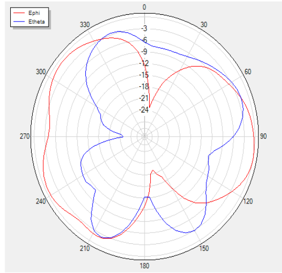
V Phi=0 freq=2020MHz
