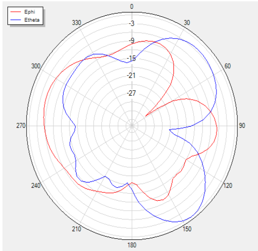
H Theta=90 freq=2360MHz
