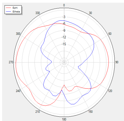
V Phi=0 freq=1720MHz
